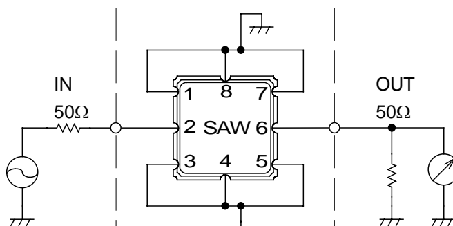
Fig.2 Measuring circuit
